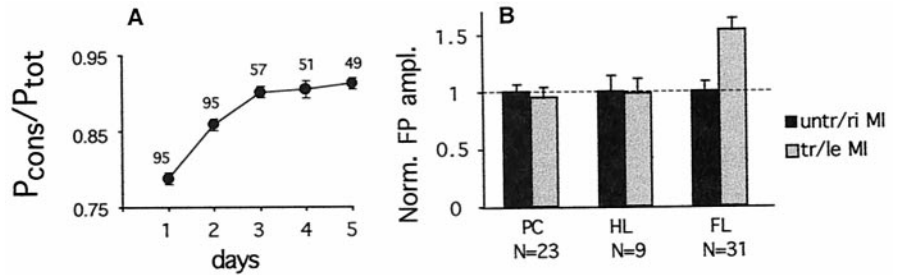
Fig. 1. Learning a new motor skill potentiates synaptic responses in MI horizontal connections. (A) Learning was defined as the success rate over time, which is the ratio of the number of consumed pellets and the number of retrieved pellets ( P_{\text{cons}}/P_{\text{tot}} \pm \text{SEM} ). Numbers above data points represent the number of animals trained for various numbers of days. A randomly chosen subset of animals trained for 5 days was used for subsequent electrophysiological recordings of the present project. (B) Learning specifically strengthened extracellular field potentials (FP) in the MI forelimb region (FL). There were no interhemispheric differences in the hindlimb region (HL) or in paired controls (PC) (12). Means \pm SEM are from four times threshold intensity (42) and were normalized to the untrained (untr) or right (ri) hemisphere. ampl., amplitude; tr, trained; le, left.
